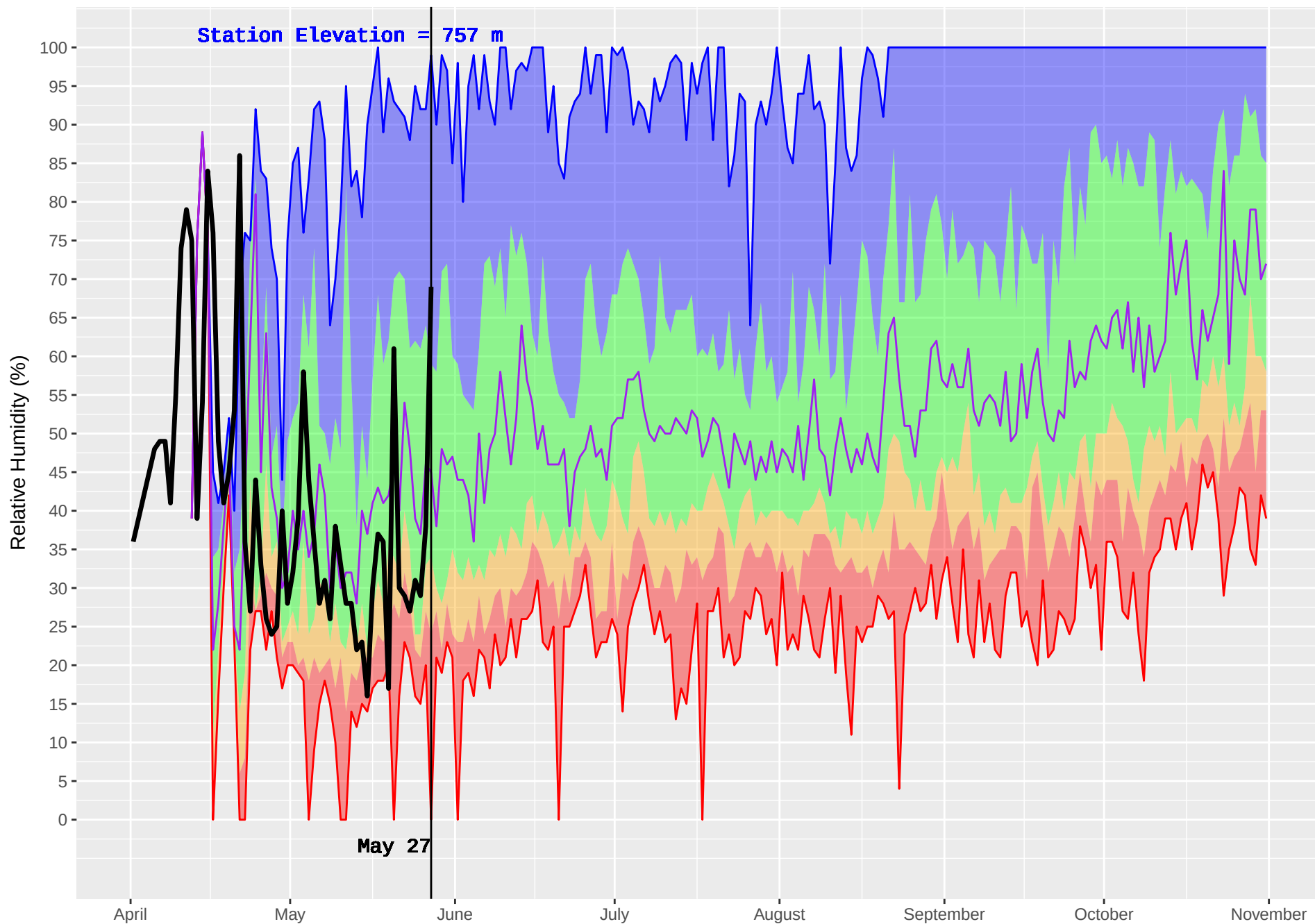
LEMORAY (140) : Historical (1988–2016) and Current (2018) Noon Relative Humidity
