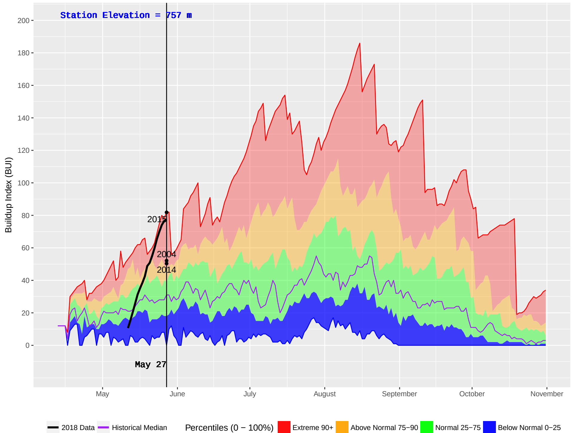
LEMORAY (140) : Historical (1988–2016) and Current (2018) Noon Buildup Index (BUI)
