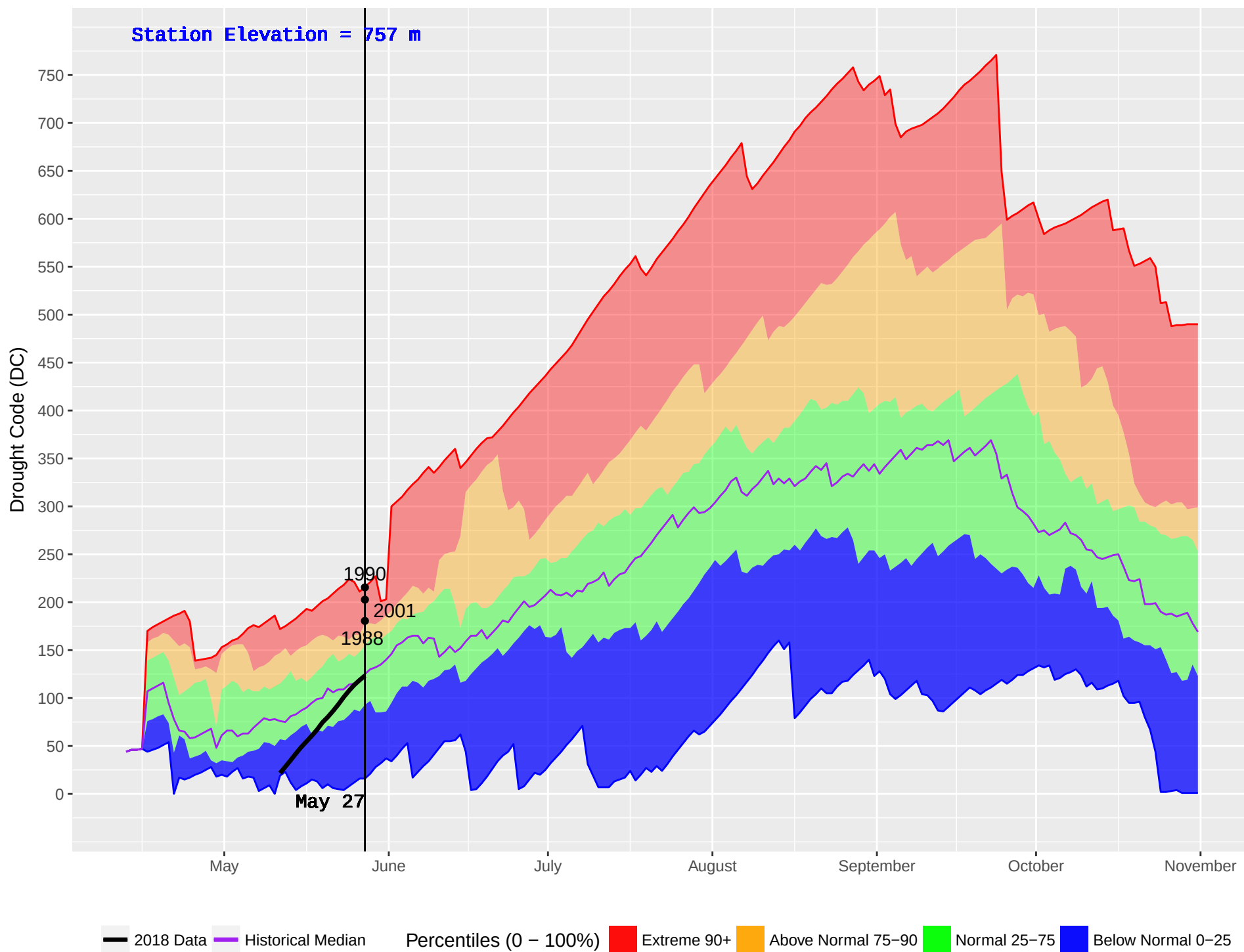
LEMORAY (140) : Historical (1988–2016) and Current (2018) Noon Drought Code (DC)
