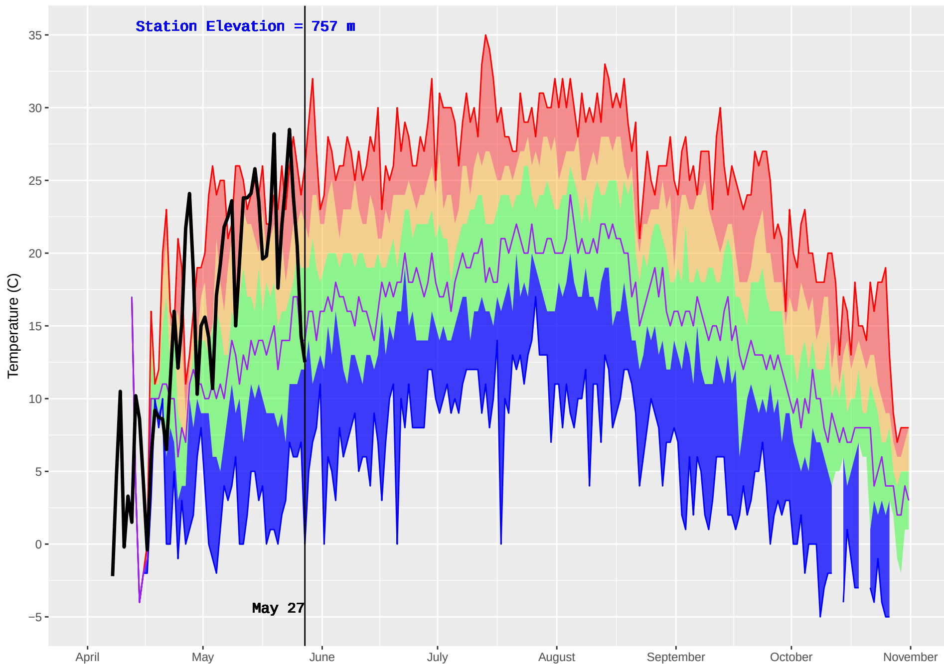
LEMORAY (140) : Historical (1988–2016) and Current (2018) Noon Temperature
